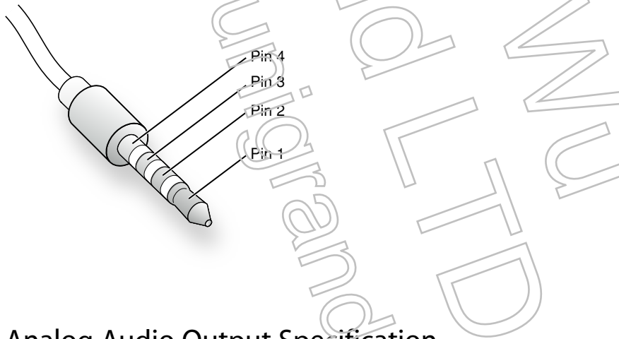
Figure 3-2 I/O plug for 2G iPod shuffle
