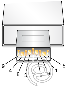
Figure 2-2 1G iPod shuffle connector
