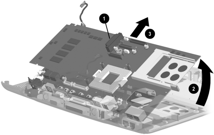
Figure 5-49. Removing the System Board
