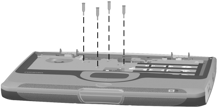
Figure C-14. Torx M2.0 × 20.0 Screw Locations
