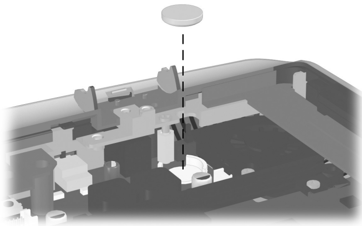
Figure 5-32. Removing the Disk Cell RTC Battery
