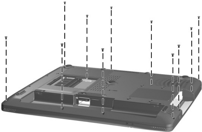
Figure C-3. Torx T8 M2.5 × 7.0 Screw Location
